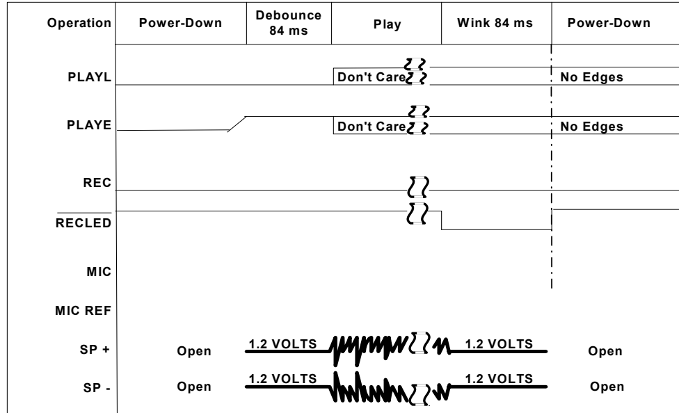
FIGURE 3: PLAY EDGE (PLAYE) PLAY UNTIL END OF MESSAGE
